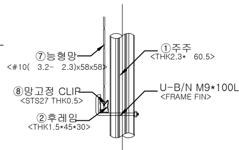
"B" DETAIL
