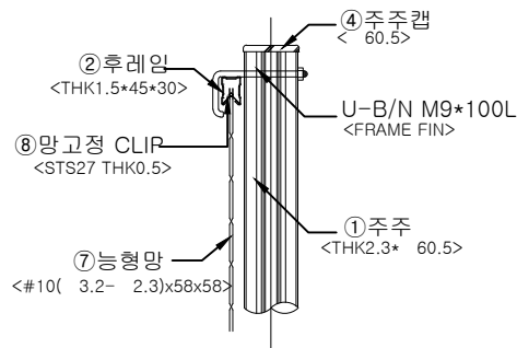
"A" DETAIL
